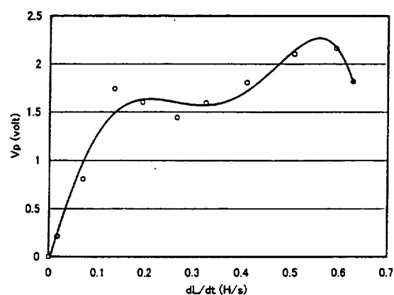
Fig. 7(b) Single coil (repulsion mode)
