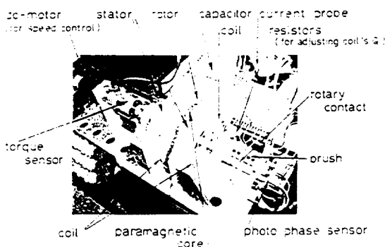
Fig. 3(a) A photograph of the whole view of the motor prototype system
