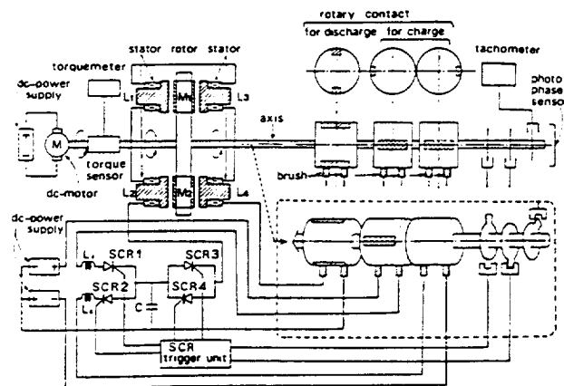
Fig. 3(b) An illustration of the configuration of the whole motor prototype system
