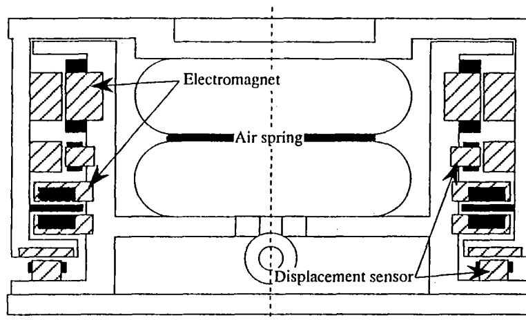
Figure 3. Cross-sectional view of electromagnetic actuator.
