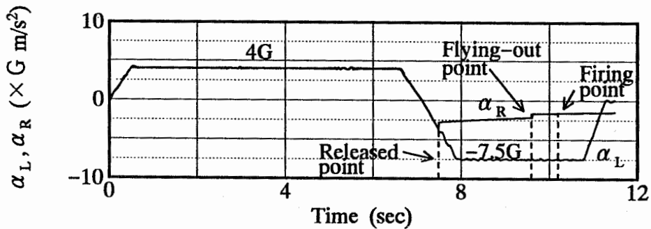
(c) Acceleration of ascending launcher and rocket
