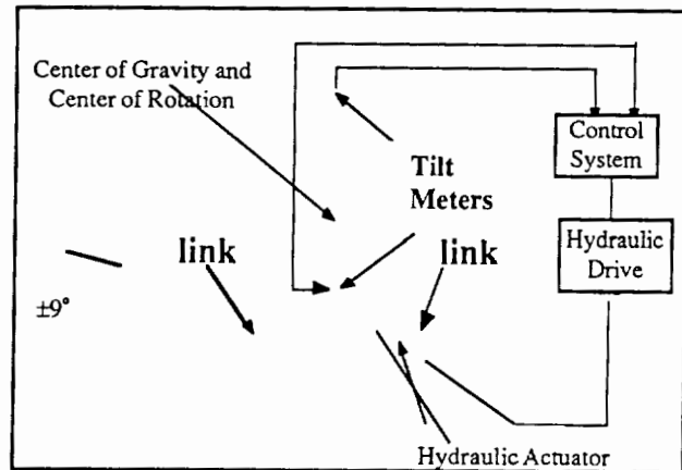
Fig. 10. Tilting mechanism and control system
