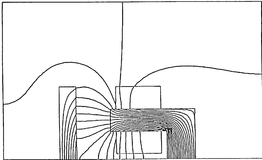
Figure 4. an example of FEM analysis results on the magnetic field of the horizontal control electromagnet with a gap of 30 mm
