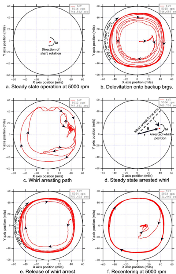
Figure 7a-f. Dropping, arresting, and releveling rotor at 5000 rpm
