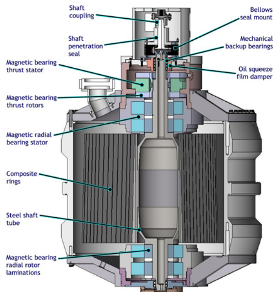
Figure 1. ALPS flywheel rotor and magnetic bearing system
