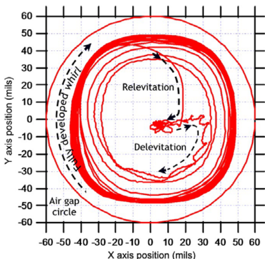
Figure 3. Bearing orbit during 2000 rpm drop test
