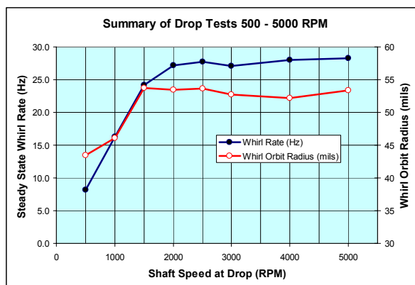
Figure 4. Whirl rates and orbits exhibited through drop tests
