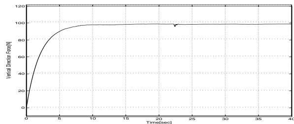
Fig. 16. Vertical Direction Force acting on the Linear Motor
