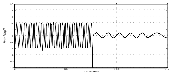
Fig. 9. Control Voltage
