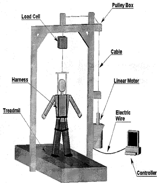
Fig. 1. Partial Body Weight Support System
