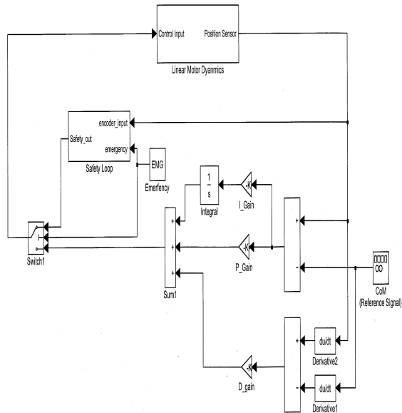
Fig. 4. Control Block Diagram
