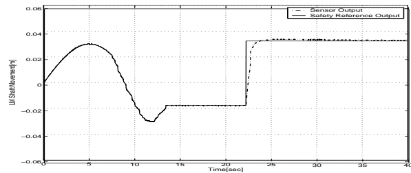
Fig. 14. Linear Motor Shaft Movement in the Safety Loop with Step Function
