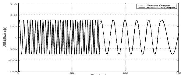
Fig. 8. Linear Motor Shaft Movement with 10[Kg] Weight
