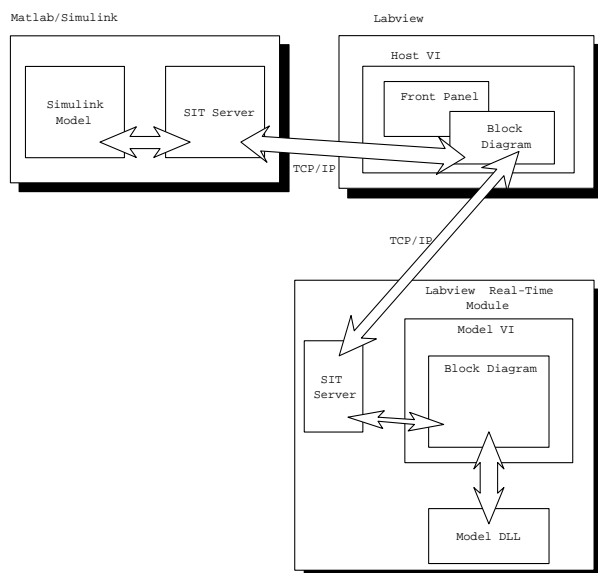
Fig. 7. Running a simulink model on an RT target
