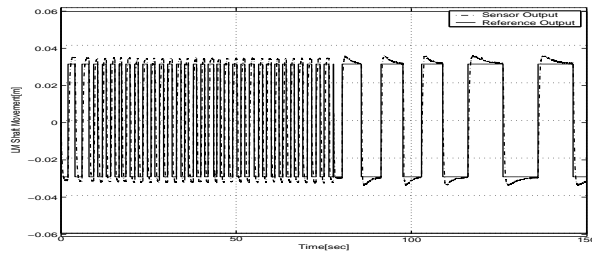
Fig. 11. Linear Motor Shaft Movement with 10[Kg] Weight
