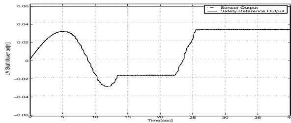
Fig. 17. Linear Motor Shaft Movement in the Safety Loop with Ramp Function
