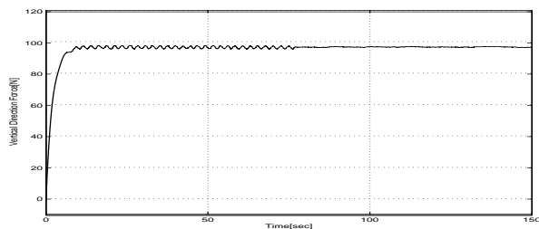
Fig. 10. Vertical Direction Force acting on the Linear Motor
