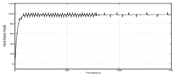
Fig. 13. Vertical Direction Force acting on the Linear Motor
