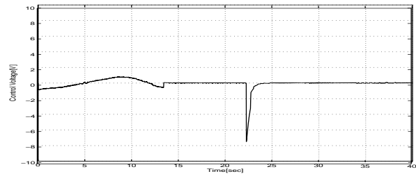
Fig. 15. Control Voltage
