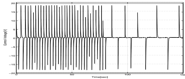
Fig. 12. Control Voltage
