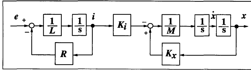
Figure 2: Nominal linear model for M.S.S.
