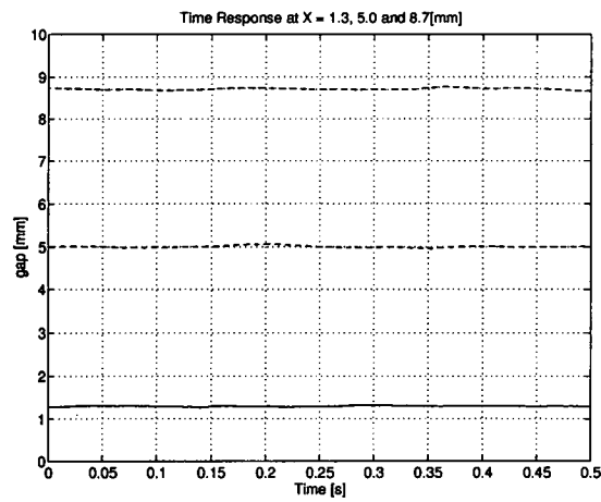
(b) Time Response at X = 1.3, 5.0, 8.7 [mm]
