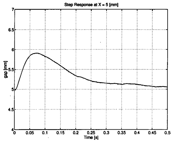
(a) Step Response at X = 5 [mm]
