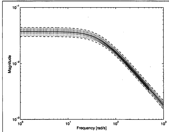
Figure 4: Frequency responses of \frac{1}{Ls+R}
