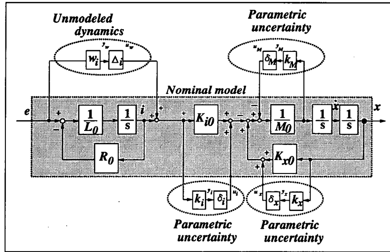
Figure 5: Set of Plant Models with Uncertainties
