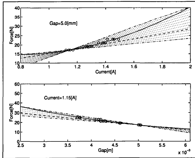
Figure 3: Current-Force Curve and Gap-Force Curve
