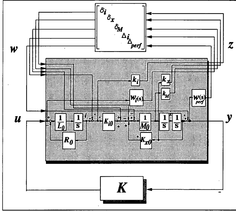
Figure 6: Interconnection Structure
