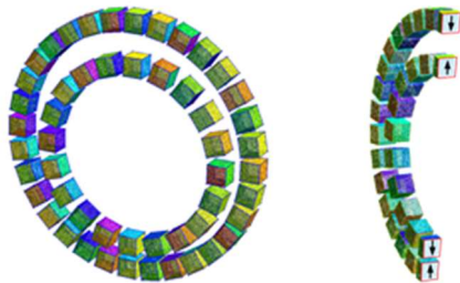
Fig. 2 One-pair configuration: one pair of magnet rings.
