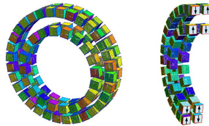
Fig. 3 Two-pair configuration: two pairs of magnet rings with repelling magnetization (inner rings: on rotor; outer rings: on stator).
