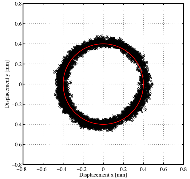
Figure 9. Trajectory of the sensorless position measurements with double sampling and symmetric voltage pulses at radial rotor displacements r=0.4\text{mm} for a setup with N_M=24 ferrite magnets (black). Rotor displacement (red).
