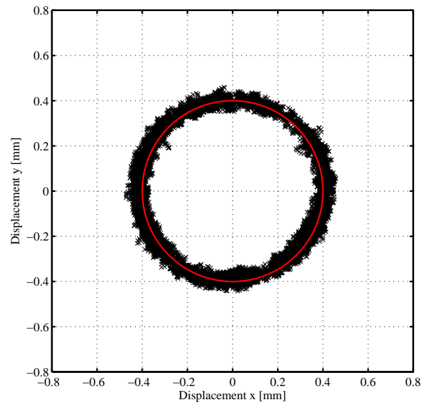
Figure 10. Trajectory of the sensorless position measurements with quad sampling and asymmetric voltage pulses at radial rotor displacements r=0.4\text{mm} for a setup with N_M=24 ferrite magnets (black). Rotor displacement (red).
