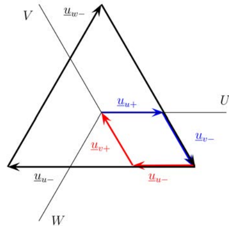
Figure 7. Voltage space phasors for three active voltage pulse injection including pre-phasors (blue) and post-phasors (red) achieving symmetric operation points
