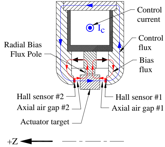
Figure 7. Structure and operational principle of the proposed electromagnetic actuator with a flux feedback.
