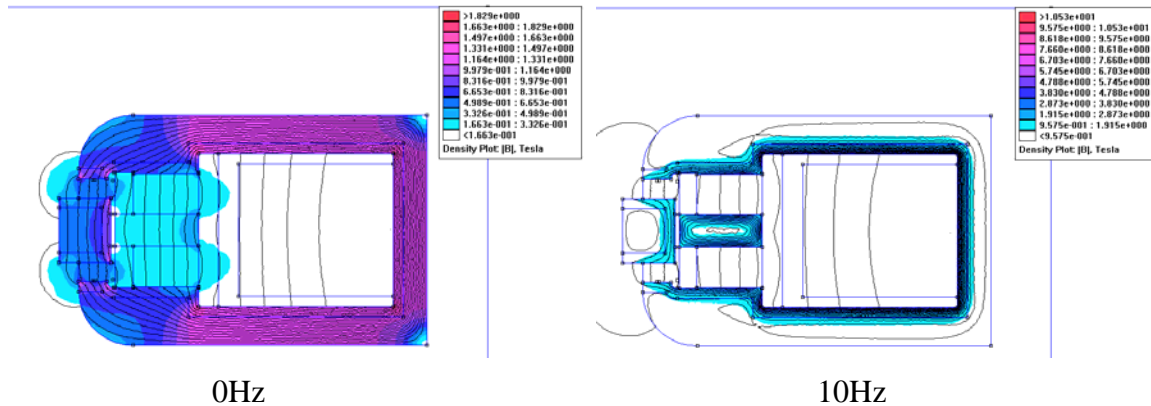
Figure 11. Control flux distribution in the actuator at 0Hz and at 10Hz.
