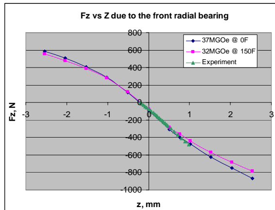
Figure 4. FEA-calculated axial force exerted on the rotor by the front AMB as a function of the axial position of the rotor ( z ) for two different combinations of the magnet strength and temperature.
