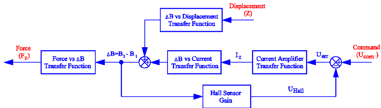
Figure 8. Control loop of the actuator with field feedback.
