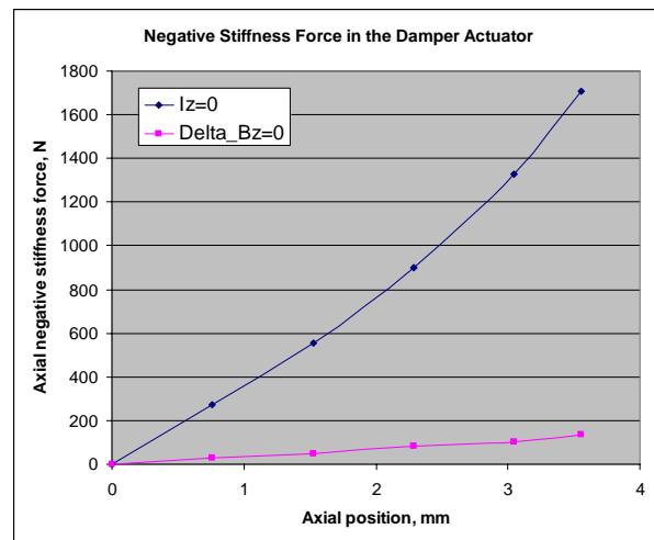
Figure 9. Comparison of the negative stiffness forces developing in the axial actuator before activating the flux feedback mode ( I_z=0 ) and after ( \Delta B_z=0 ).
