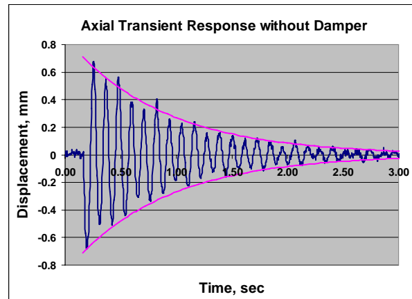
Figure 5. Axial rotor oscillations in a standalone motor following a hammer impact.
