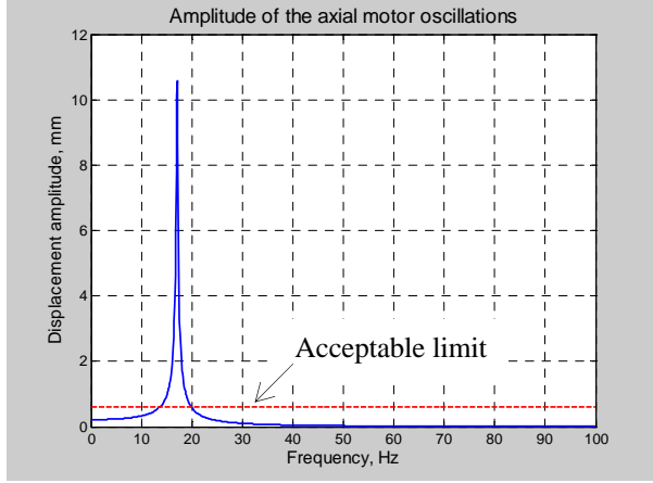
Figure 6. Axial frequency response of the motor rotor to the axial oscillations of a compressor rotor with 0.25mm amplitude and the axial damping equal to 1% of the critical damping.
