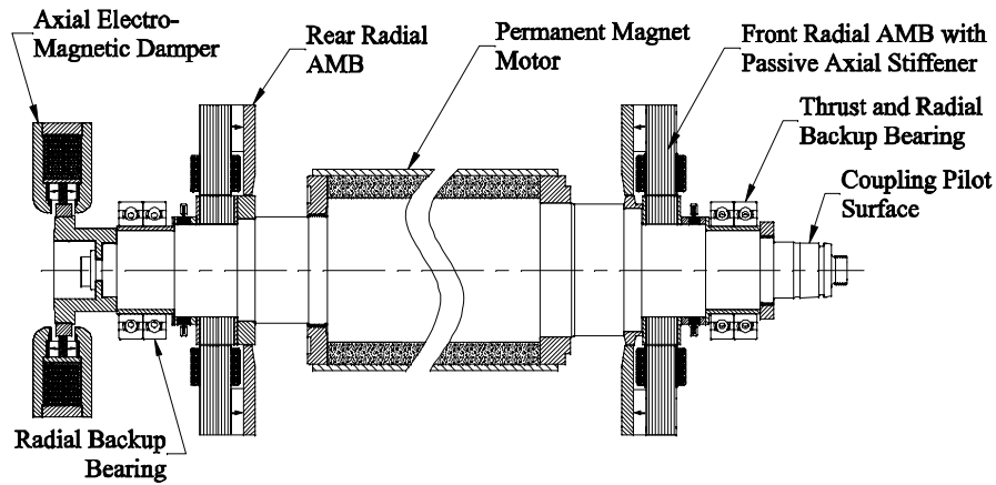
Figure 2. Layout of a 1MW 15kRPM motor on magnetic bearings.
