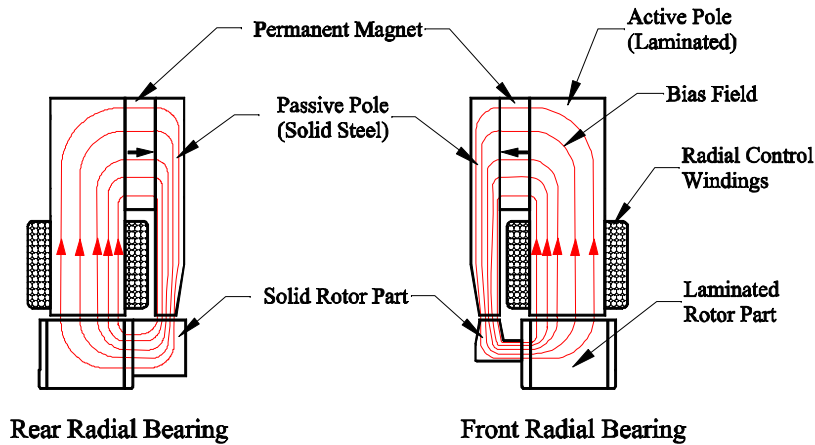
Figure 3. Bias flux distribution in the front and rear radial bearings.
