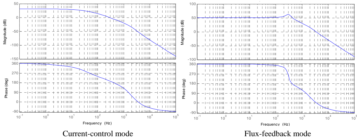
Figure 12. Actuator transfer functions in the current-control mode and the flux-feedback mode.
